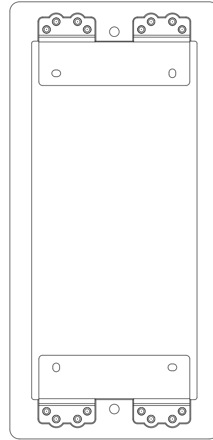
4 BACK VIEW
