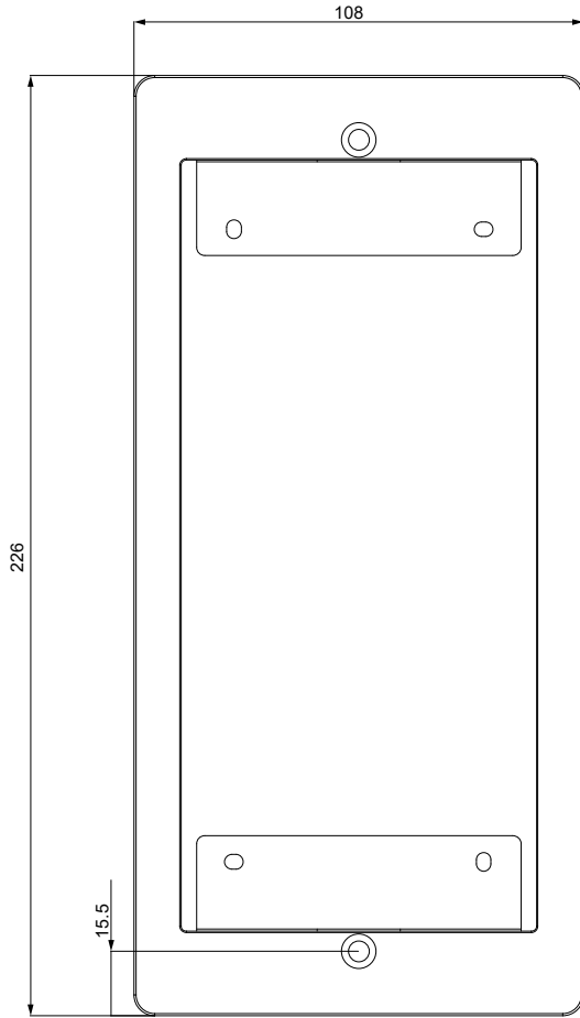
1 FRONT VIEW
