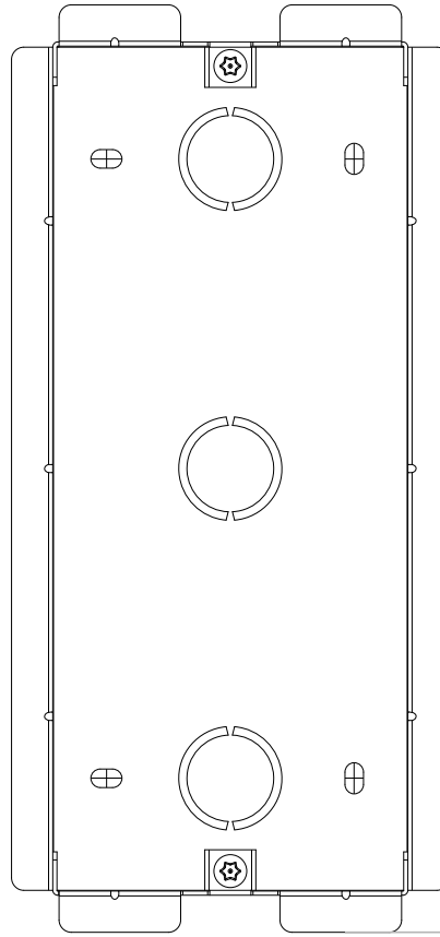
2 FRONT VIEW: FLUSHING MOUNTING BOX PLACEMENT
