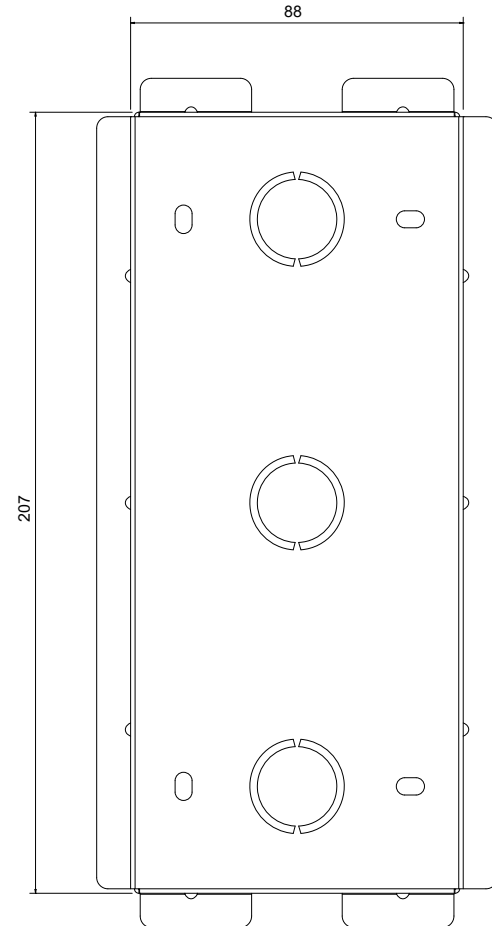
4 BACK VIEW
