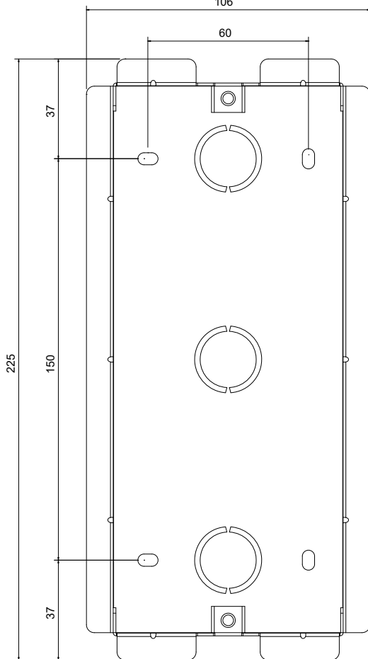
1 FRONT VIEW
